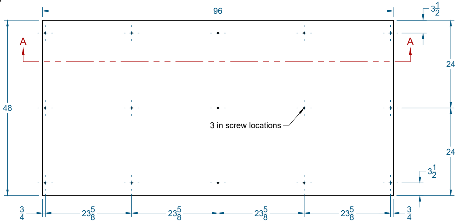
Top view
