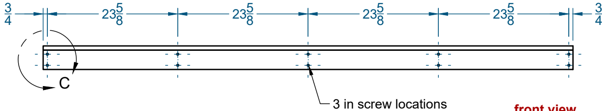
front view
